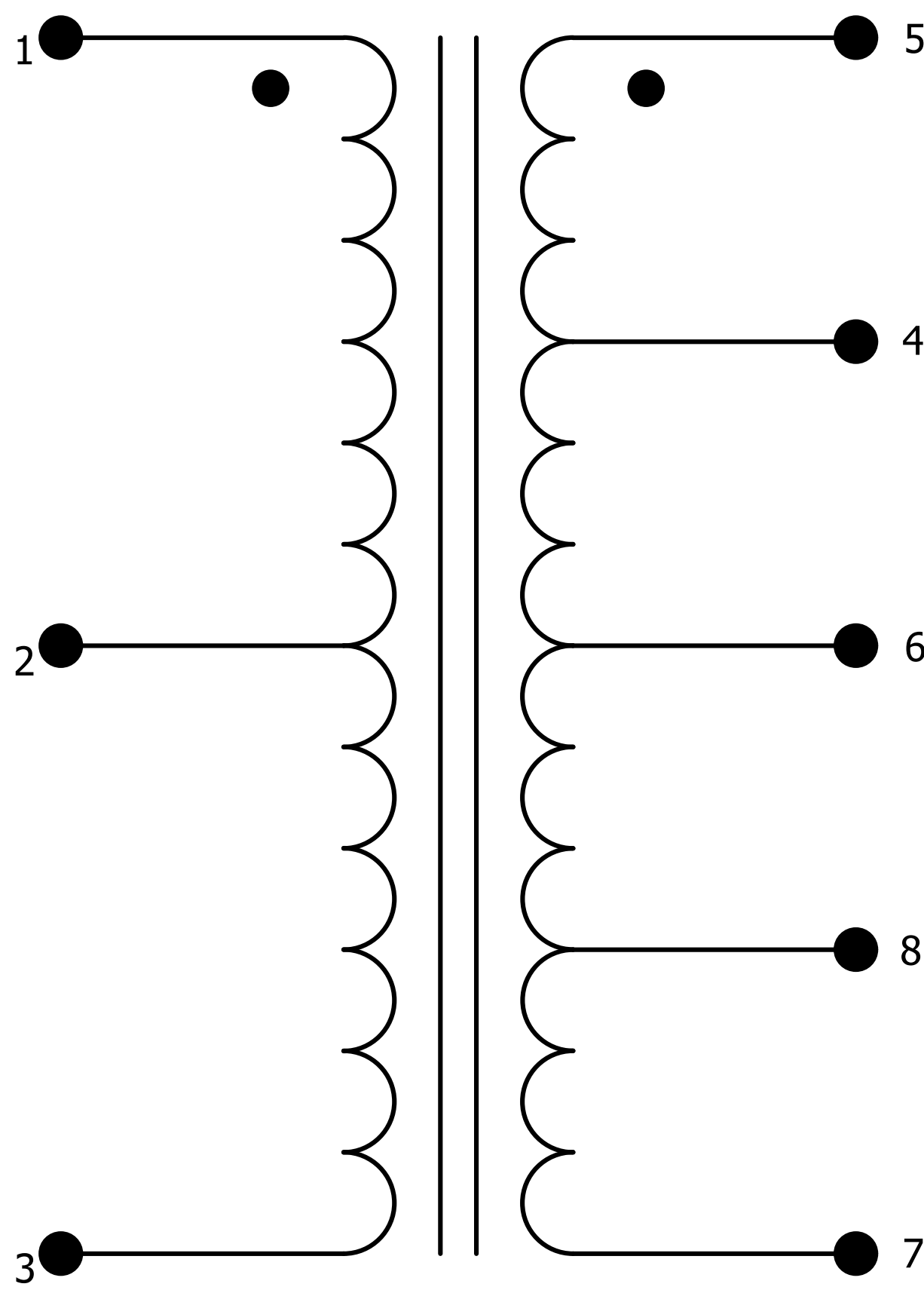
CIRCUIT DIAGRAM FOR DASH NUMBER 04
