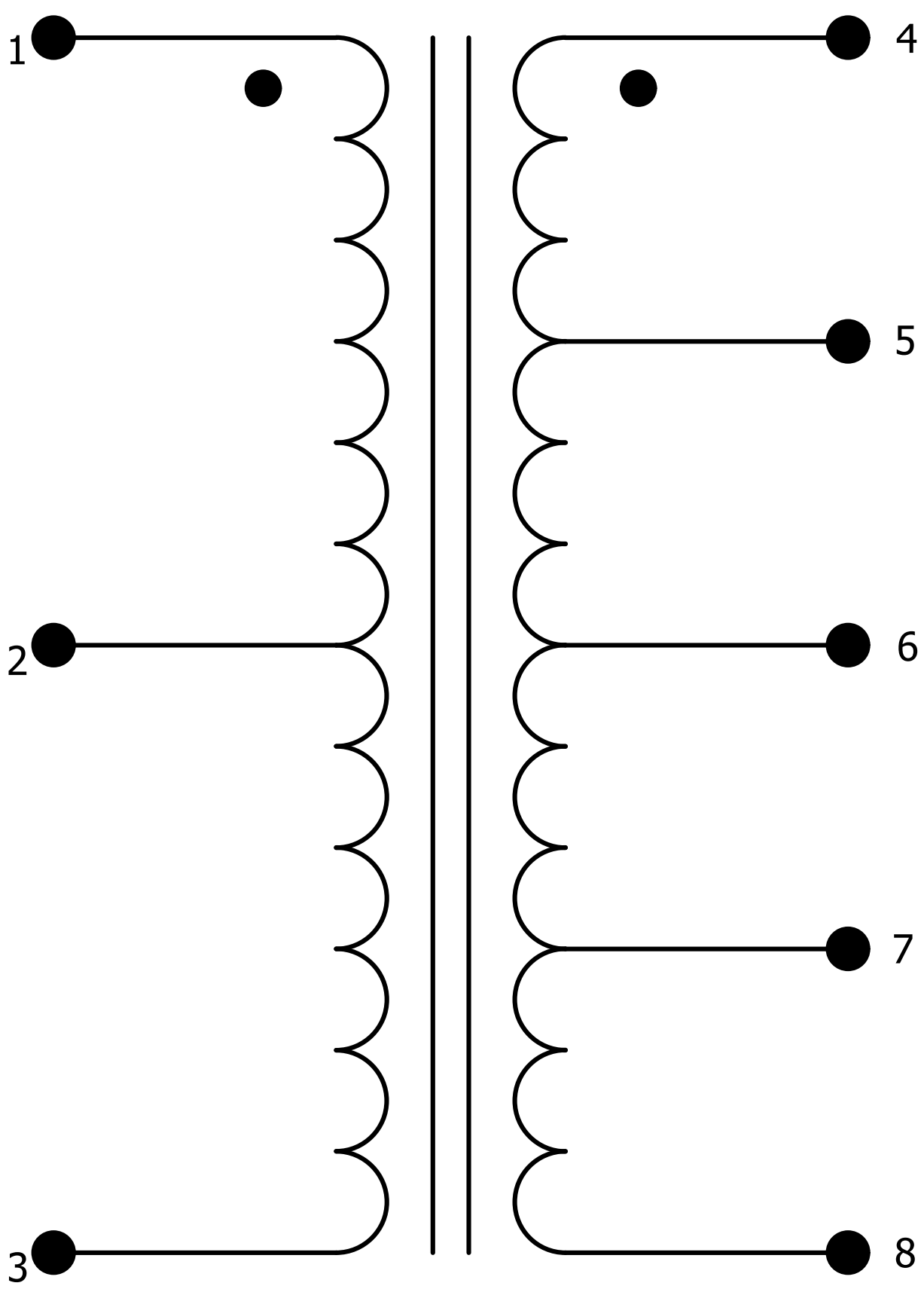
CIRCUIT DIAGRAM FOR DASH NUMBERS 01, 02, 03, 10, AND 26
